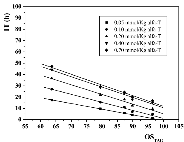
Figure 5. Relationship between the induction time (IT) and oxidative susceptibility ( OS_{TAG} ) of matrices with different triacylglycerol compositions spiked with different concentrations of \alpha -tocopherol ( \alpha -T).
